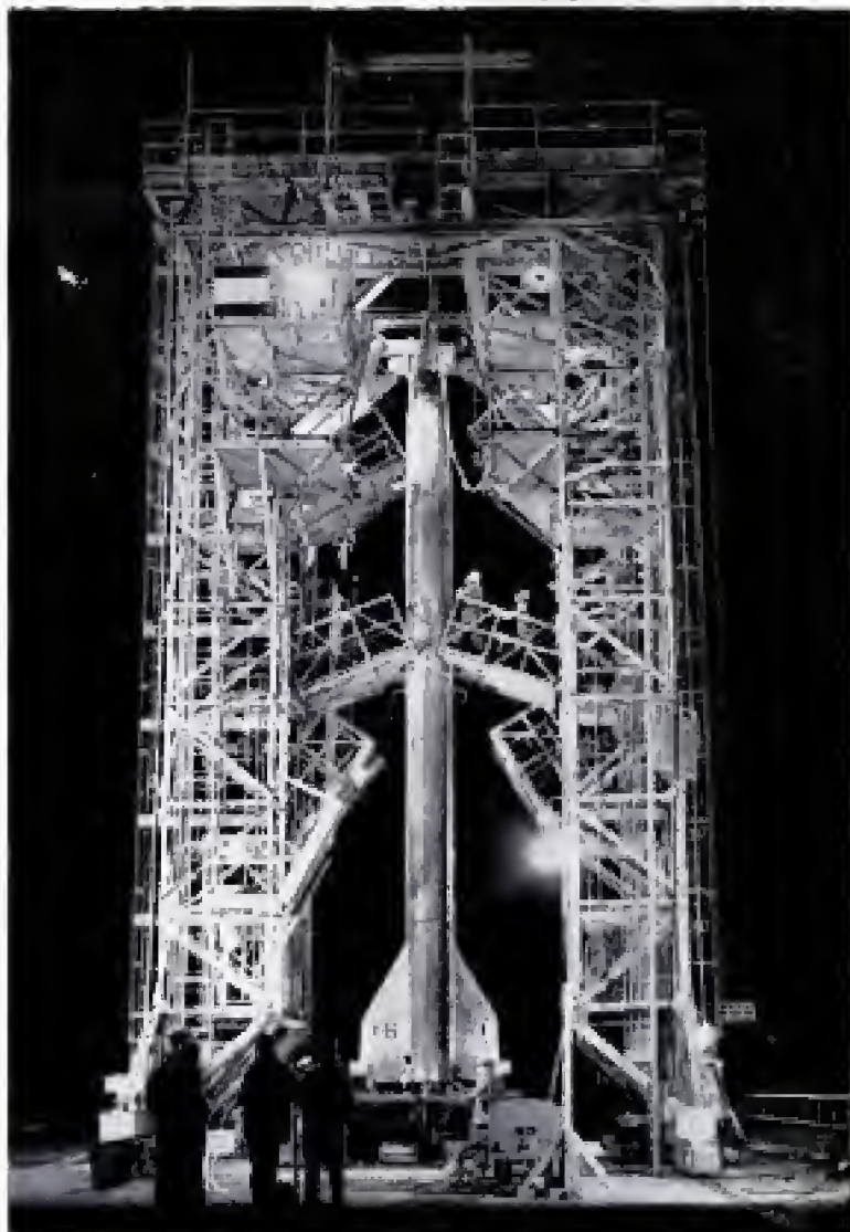
Elaborate scaffolding is required for launching of Viking high altitude research rocket at the White Sands Proving Ground, N. M.
